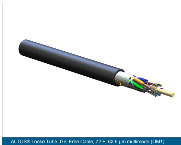
ALTOS® Loose Tube, Gel-Free Cable, 72 F, 62.5 μm multimode (OM1)
